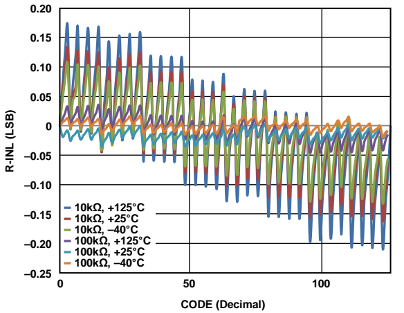
Figure 7. R-INL vs. Code (AD5122A)
