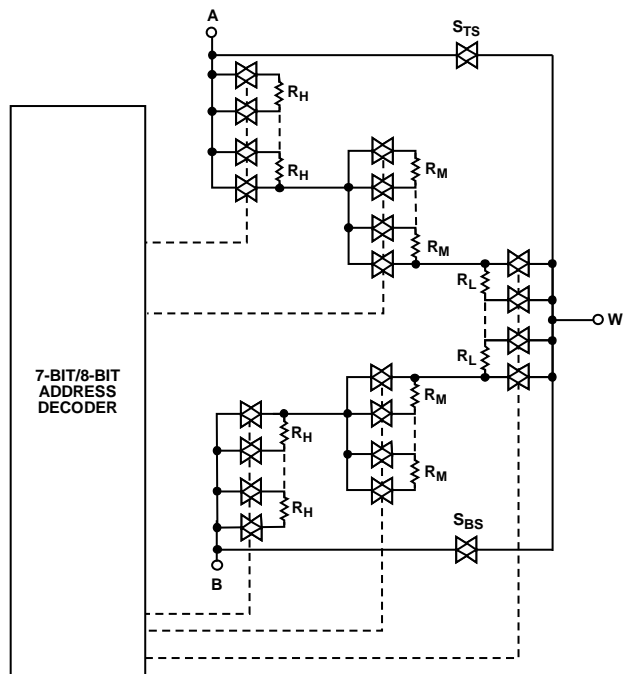
Figure 37. AD5122A/AD5142A Simplified RDAC Circuit
